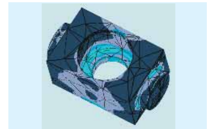
STRESS ANALYSIS OF HOOK CROSS - HEAD
