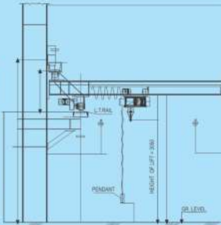
TRAVELLING CANTILEVER WALL TYPE JIB CRANE
