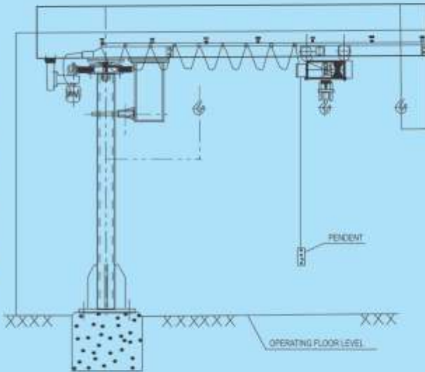
PILLAR MOUNTED JIB CRANE WITH 270°/360° SWIVELLING
