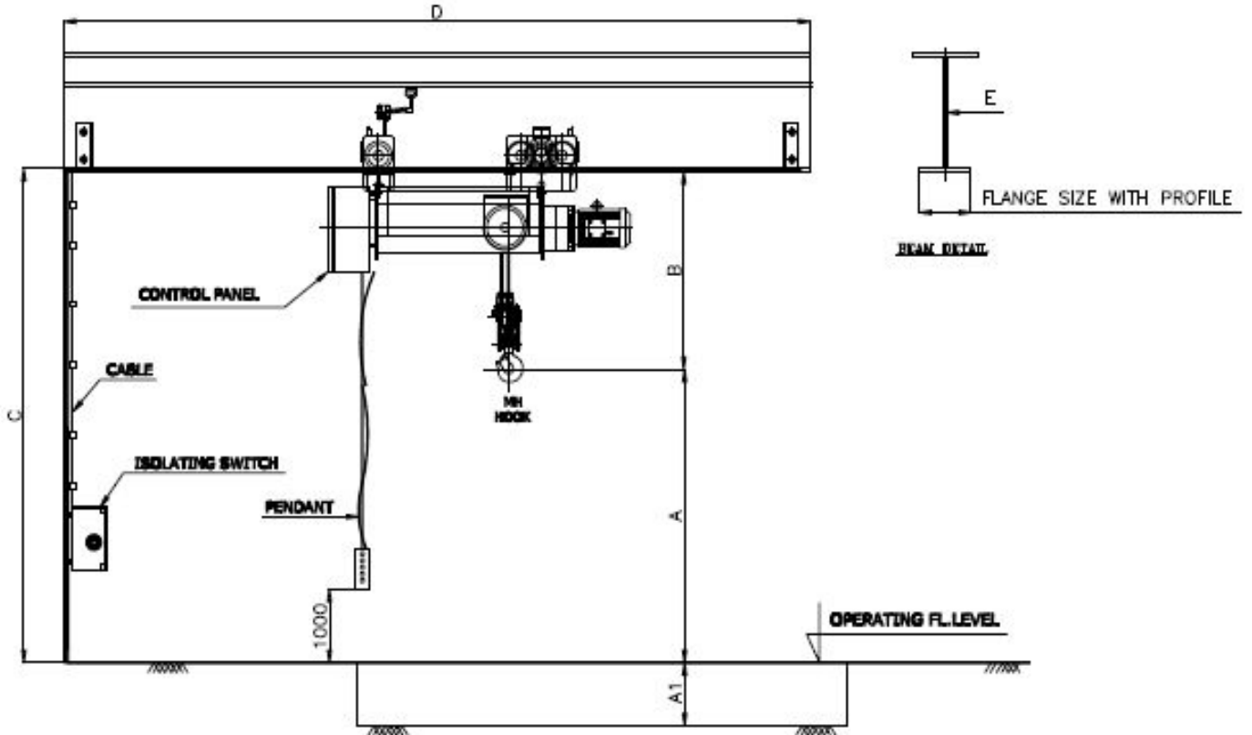
CLEARANCE DIAGRAM ELECTRIC WIRE ROPE HOIST
