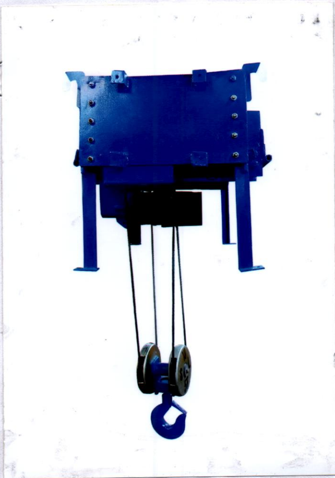
RIGHT VIEW
