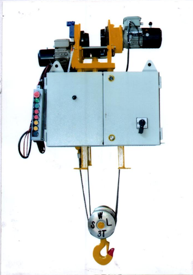
RIGHT VIEW
